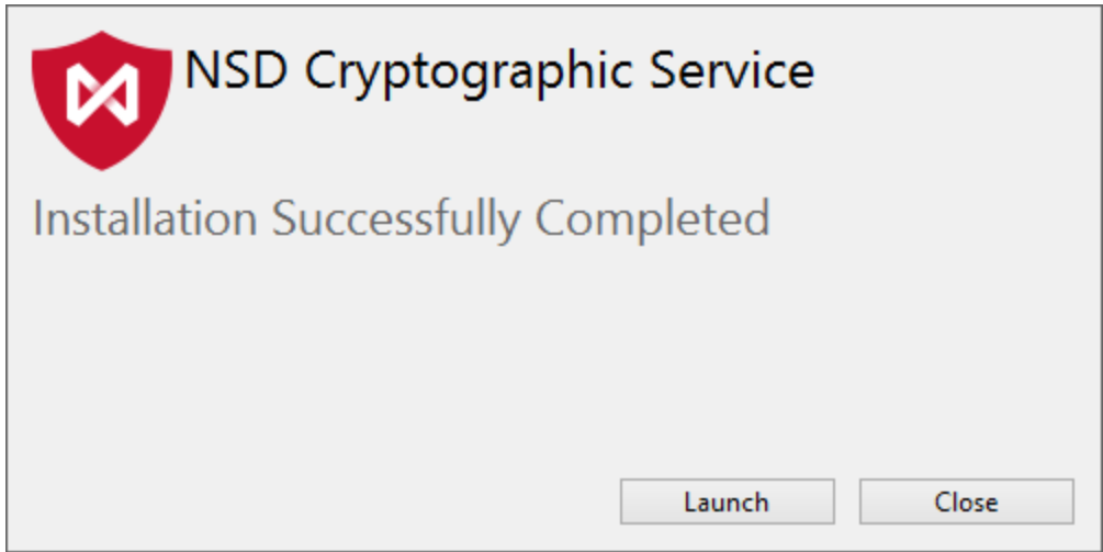
Figure 3 – completing installation
