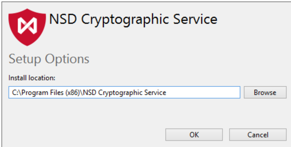
Figure 2 – installation folder
