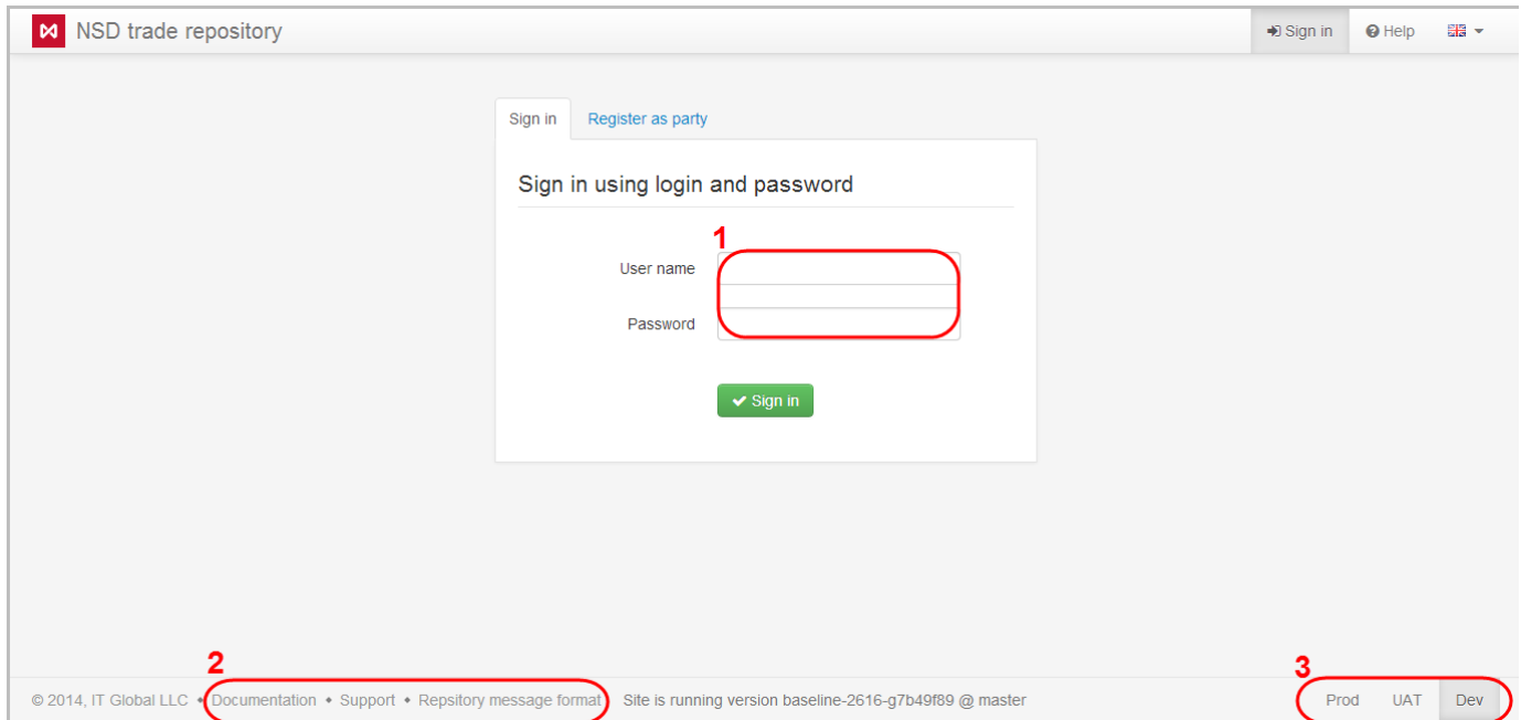
Fig. 1 – user Authentication
