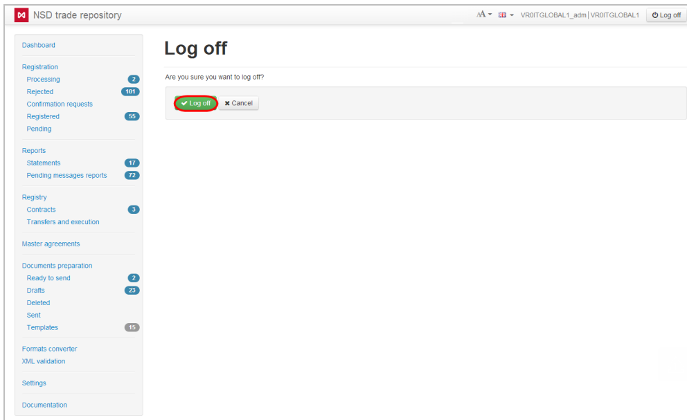
Fig. 3 – logout confirmation
